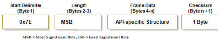
Figure 5-01. UART Data Frame Structure
